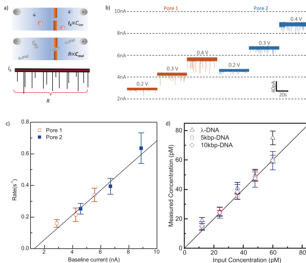
Figure 5. (a) Schematic of ions and molecules translocation through the same nanopore. The ion and molecule translocation rate is experimentally obtainable from the continuous current readout. (b) Current time trace of 24 pM 10 kbp DNA (in 1 M KCl) translocating through two different nanopores under different voltages. (c) The molecule translocation rate is linearly proportional to the baseline current for the same test sample shown in (b). (d) Validation of the calibration-free method for concentration determination. The test was performed with different nanopores and DNA molecules with different sizes.
