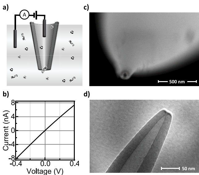
Figure 2. Experimental setup and nanopore characterization. (a) Illustration of the experimental setup (not to scale). Ag/AgCl electrodes were inserted to the nanopore and bulk solution to apply the bias voltage across the nanopore. (b) A typical IV curve for glass nanopore in 1 M KCl with Tris-EDTA-buffer solution. (c) SEM image of the glass nanopore showing the overall shape. (d) The TEM image of the nanopore tip showing apparent conical shape.
