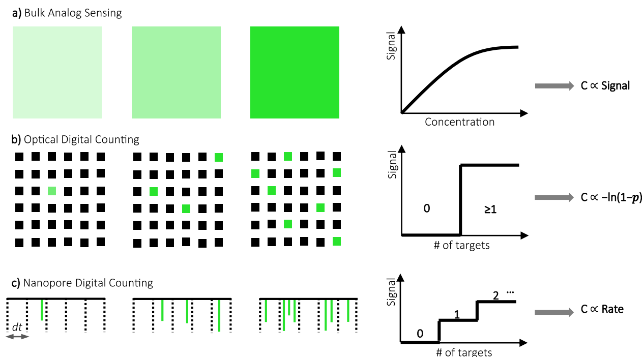
Figure 1. Comparisons for different quantification methods. (a) Analog sensing generates a signal proportional to the bulk sample concentration. (b) In the optical digital counting, the sample is partitioned into many small containers such that each partition contains a discrete number of biological entities. The sample concentration is determined by Poisson statistics ( p is the positive ratios). (c) In nanopore digital counting, the sample concentration is proportional to the single molecule translocation rates.
