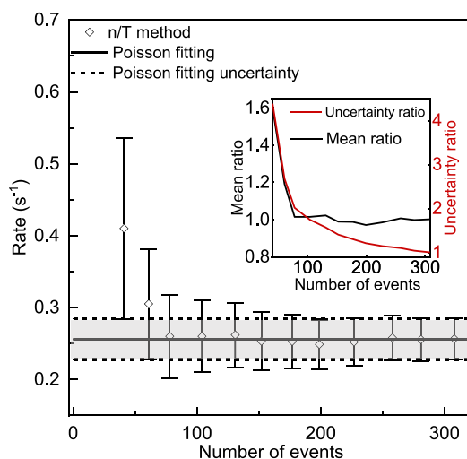
Figure 4. Translocation rate determined by the n/T method for increasing the observation numbers. The shaded area is the value obtained by the Poisson fitting method (mean + uncertainty). The inset shows the mean and uncertainty value comparison between these two methods.
