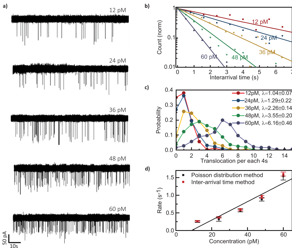
Figure 3. Translocation recording of \lambda -DNA through glass nanopore at 1 M KCl under 400 mV bias. (a) Continuous current readout illustrating the translocation events at different DNA concentrations. The average molecular distance is around 3 \mu m, the interactions between molecules are negligible. (b) Normalized distributions of interarrival time for different concentrations with monoexponential fits to the distributions. (c) The probability distribution of the events for different concentrations. The 4 s time interval is used to better show the Poisson distribution. (d) The translocation rate obtained from both fitting methods versus the \lambda -DNA concentrations.
